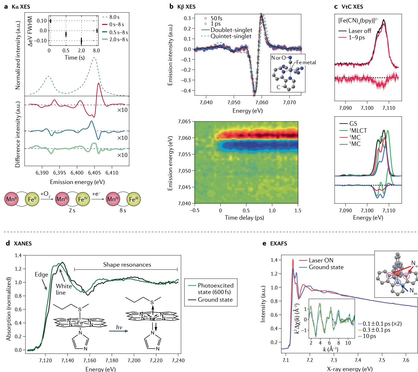
Fig. 2 | Hard X-ray spectroscopy at X-ray free-electron lasers. a | Fe Kα X-ray emission spectroscopy (XES) of solutions of Fe/Mn containing ribonucleotide reductase R2c measured at room temperature prior to O 2 incubation, and changes observed after 0.5, 2 and 8 s in situ O 2 incubation. The change in spectral shape and full width at half maximum (FWHM) indicates, first, formation of a Fe IV intermediate (within ~2 s), followed by the catalytically active Fe III state (schematic). b | Transient Fe Kβ XES difference spectra of Fe(CN) 4 (bpy) (bpy = 2,2'-bipyridine; structure in inset) at 50 fs and 1 ps after photoexcitation and the calculated difference involving either a doublet metal–ligand charge transfer (MLCT) or a quintet metal-centred excited state (top). The contour plot (bottom) shows light-induced changes of the XES up to 1.5 ps after excitation. The spectra indicate that, likely, only one excited state is present and the MLCT state fits the data best. c | Transient Fe valence-to-core (VtC) XES of Fe(CN) 4 (bpy) (top) and calculated spectra (bottom), showing light-induced changes in the picosecond time range due
