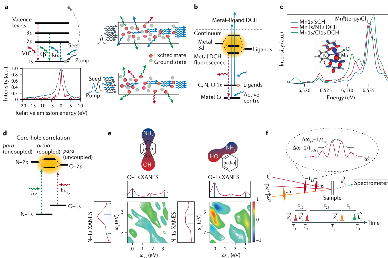
Fig. 5 | Examples of future X-ray free-electron laser-based nonlinear spectroscopy methods. a | Level diagram of various transition-metal K emission lines (top left) and schematics of amplified spontaneous emission (top right) and seeded stimulated emission (bottom right). The pump pulse is tuned above the K-edge to create 1s core-hole excited states in the sample (red dots). In amplified spontaneous emission, a randomly forward emitted photon stimulates emission when encountering an excited atom, leading to amplification along the path of atoms in the excited state, as created by the pump pulse. In seeded stimulated emission, the seed pulse energy is tuned to that of the emission line that one wants to enhance along the pump or seed pulse direction. Single-shot seeded K \beta stimulated X-ray emission spectroscopy (S-XES) spectrum (red line) of NaMnO 4 compared with conventional X-ray emission spectroscopy (XES) spectrum (blue line), showing the potential for spectral narrowing in S-XES (bottom left). b | Level diagram and calculated valence-to-core (VtC) spectra in metal–ligand double-core-hole XES. Two photons from the X-ray free-electron laser pulse simultaneously create a double-core-hole (DCH) state, with one core-hole in the metal and one in the ligand. c | Calculated DCH spectra with N and Cl
